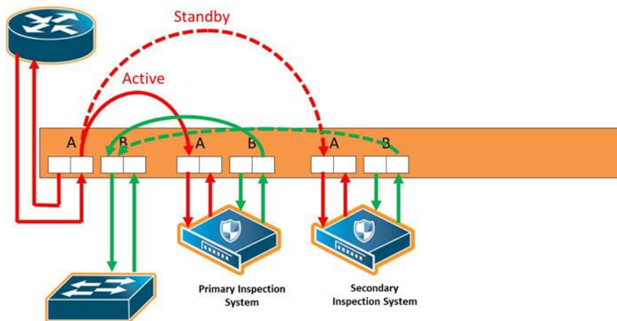
Figure 75 Inline Tool Group With Spare, Redundant 1+1 Scenario
