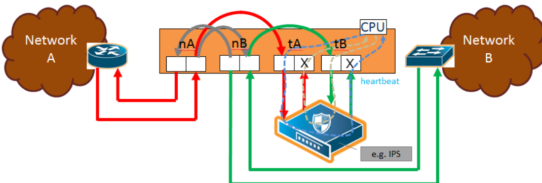
Figure 67 Traffic Path of Monitoring
