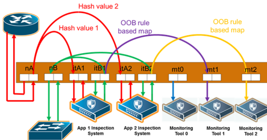
Figure 93 Out-of-Band Rule-Based Maps
