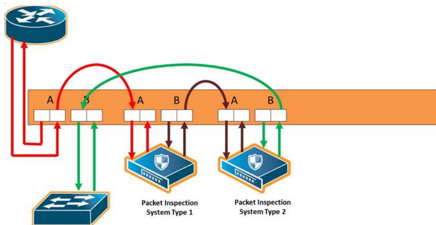
Figure 61 Inline Tool Series
