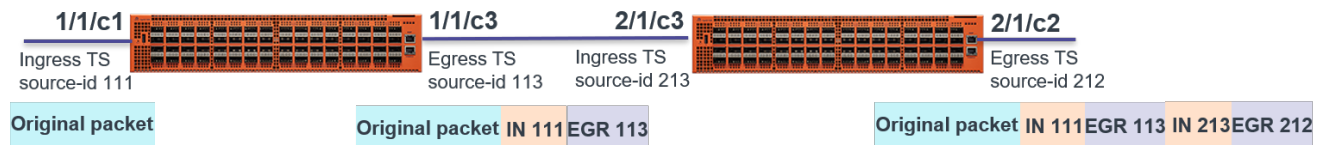
Figure 101 Timestamping
