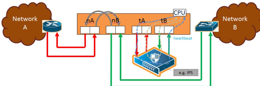
Figure 66 Traffic Path of Bypass
