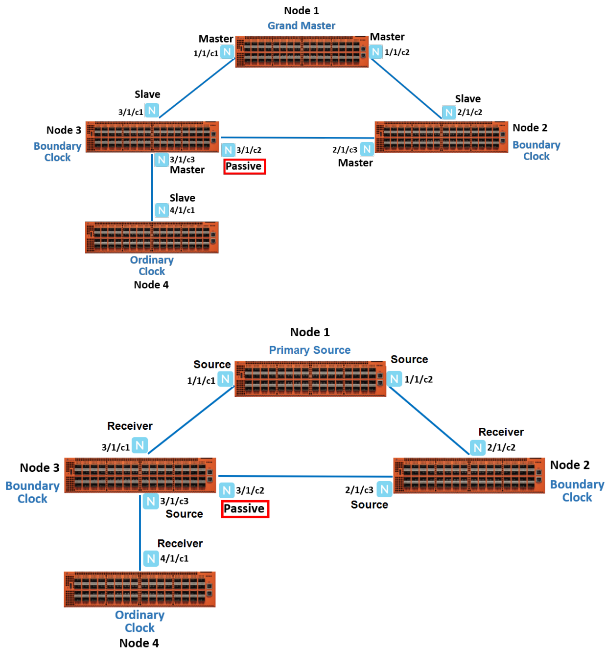
Figure 102 PTP Deployment
