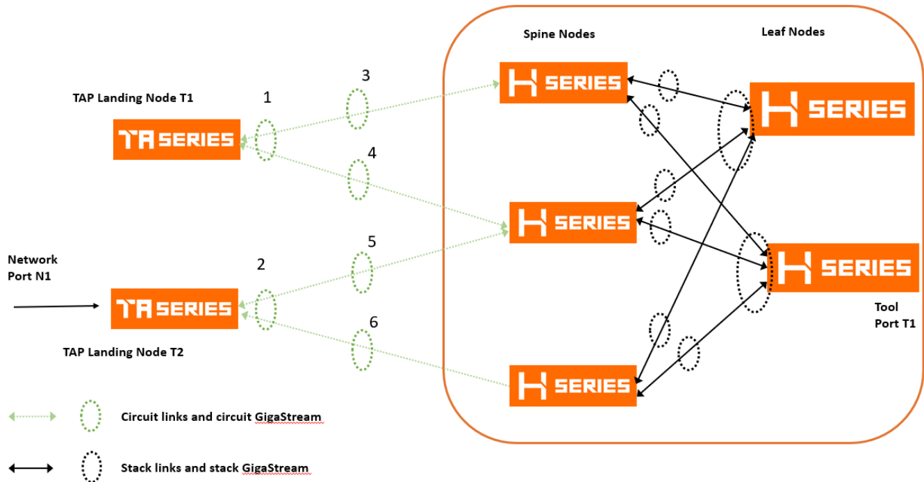
Figure 112 Leaf-Spine Based Topology.
