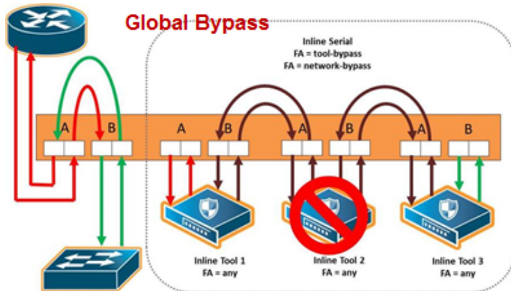
Figure 80 Inline Tool Series Global Bypass Failover Action
