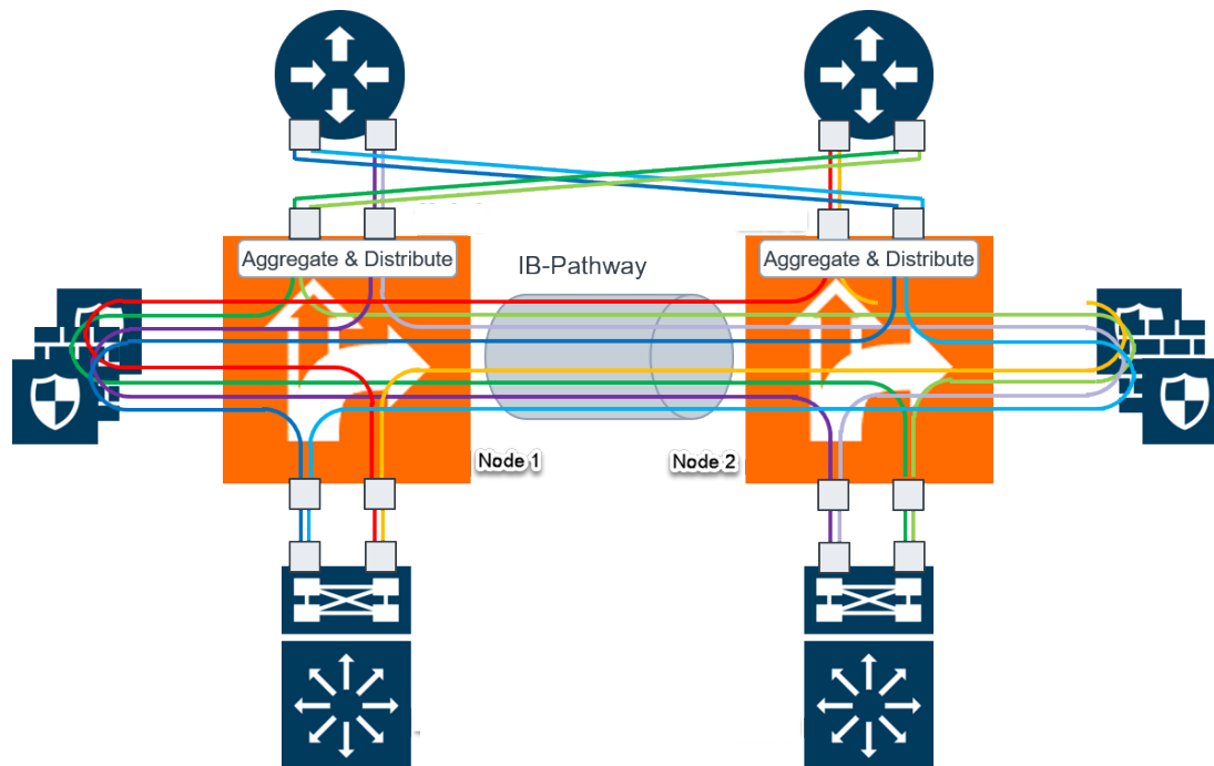
Figure 53 Resilient Inline Arrangement
