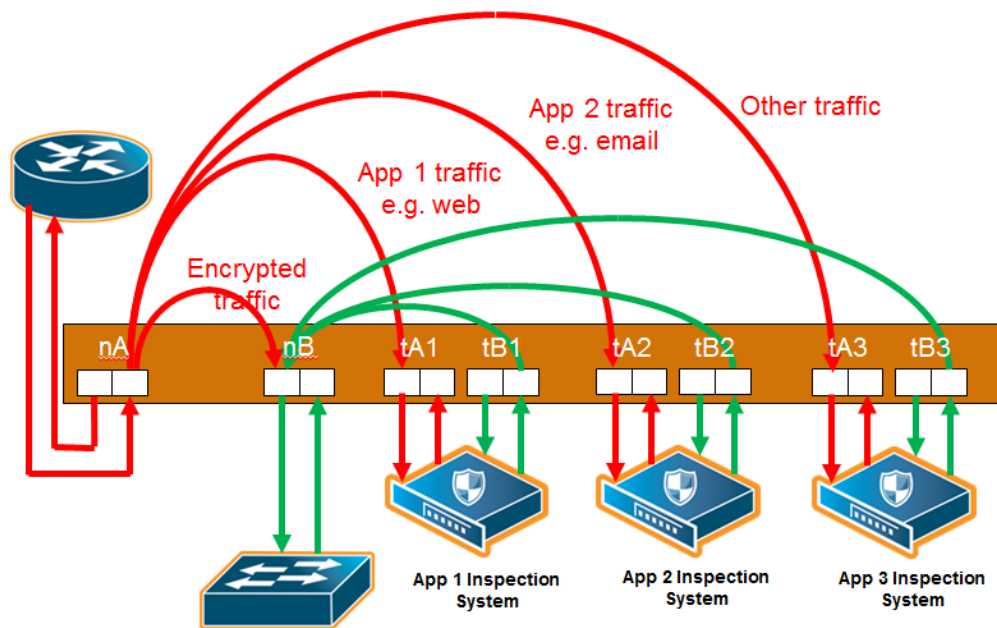
Figure 63 Inline Flow Mapping® Based Traffic Distribution
