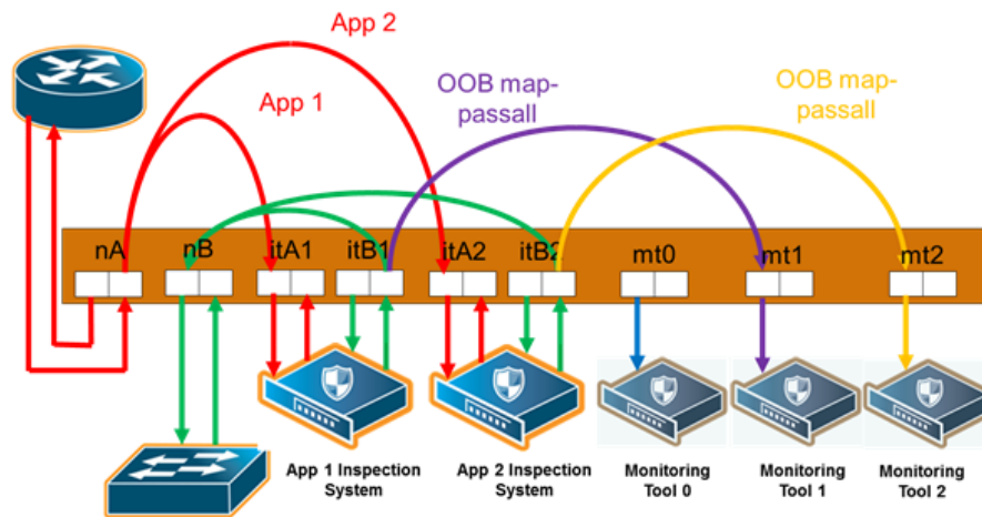
Figure 94 Out-of-Band Map Passalls
