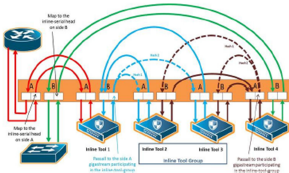
Figure 79 Inline Tool Series, Including Inline Tool Group
