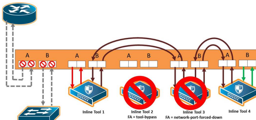
Figure 88 Inline Tool Series Local Failover of Two Tools
