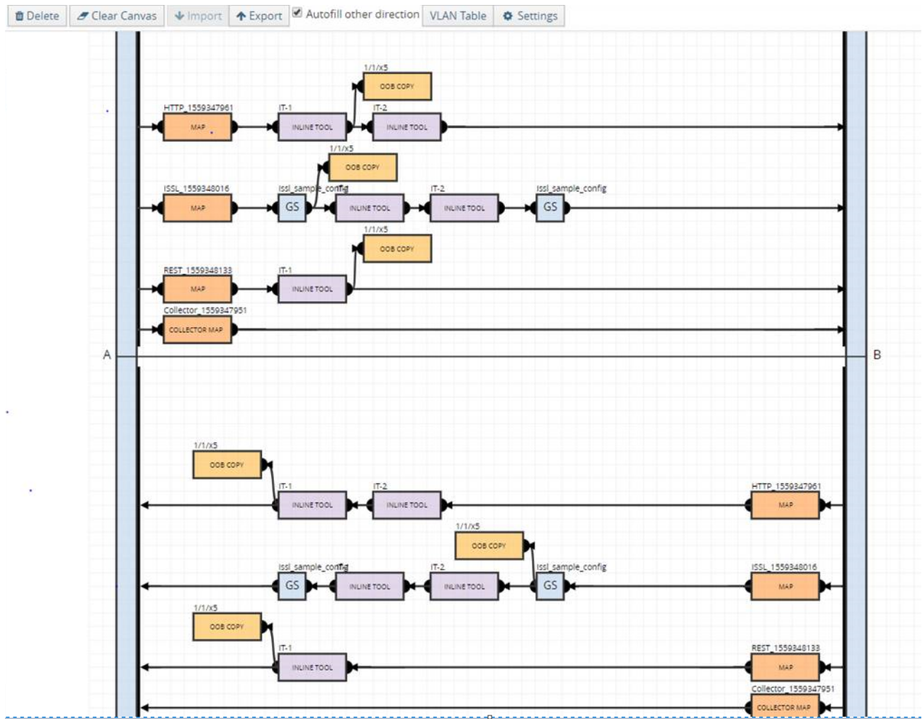
Figure 56 Flexible Inline SSL APP—Deployed
