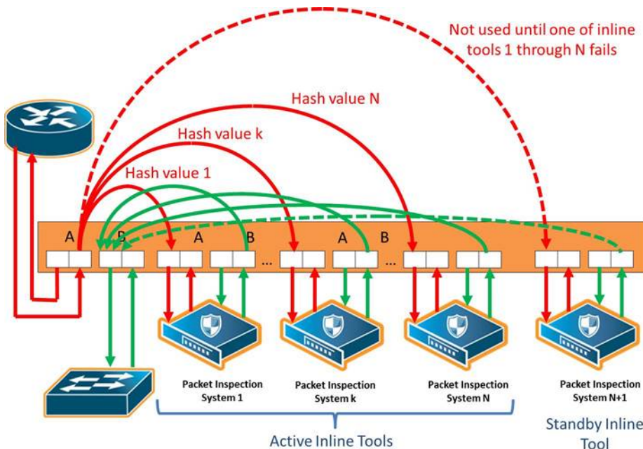
Figure 76 Inline Tool Group With Spare, Redundant N+1 Scenario
