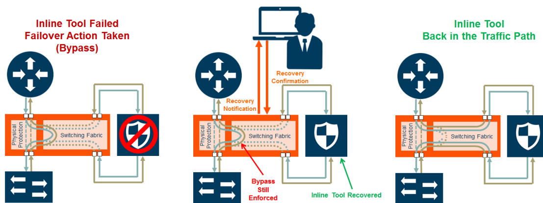
Figure 72 Automatic and Manual Inline Tool Recovery from Failover
