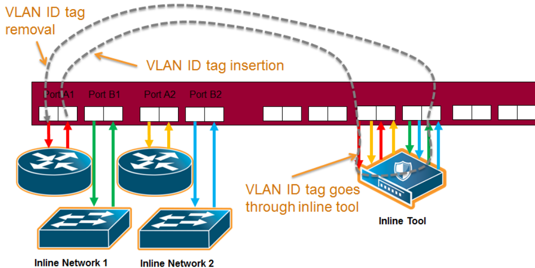
Figure 69 Inline Network Group Many-to-One
