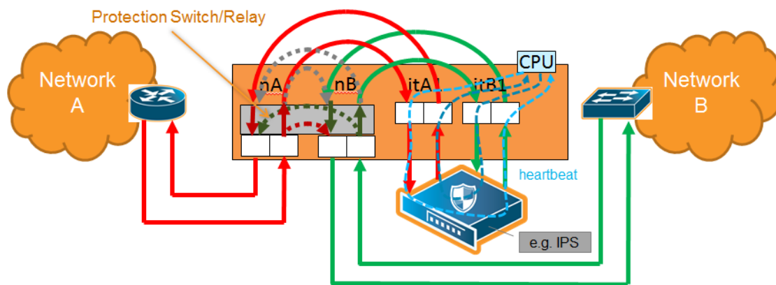
Figure 58 Physical Bypass Protection
