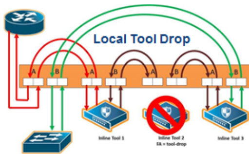
Figure 84 Inline Tool Series Local Tool Drop Failover Action
