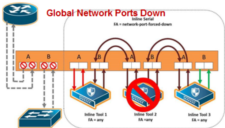
Figure 81 Inline Tool Series Global Network Ports Forced Down Failover Action
