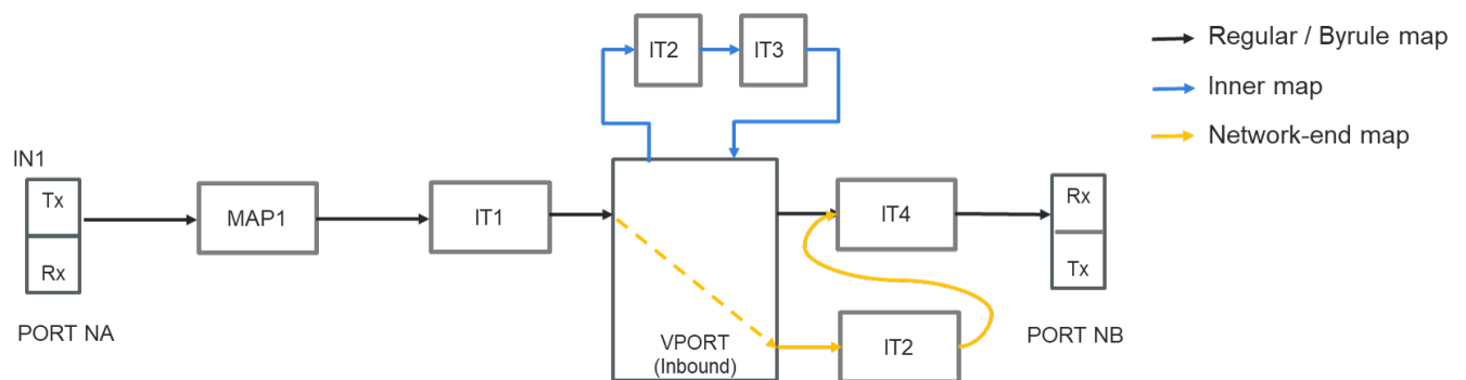
Figure 55 Flexible Inline Decryption Maps
