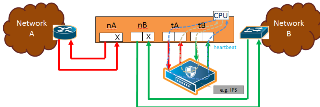
Figure 65 Traffic Path of Drop
