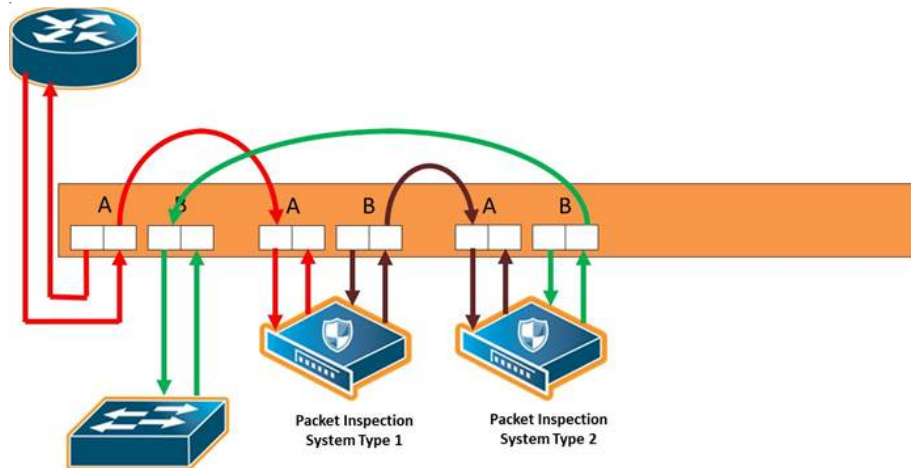
Figure 78 Inline Serial Tools
