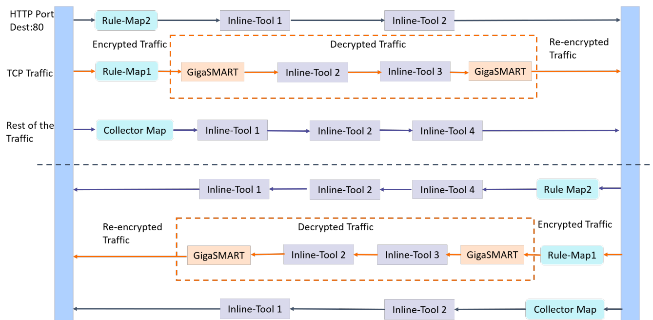
Figure 54 Flexible Inline Decryption Solution
