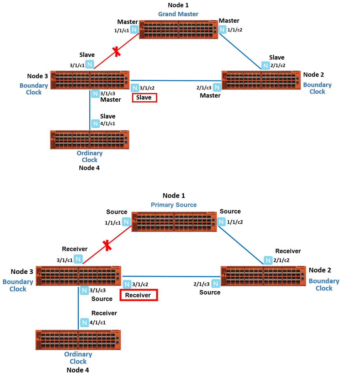
Figure 103 PTP State Transition
